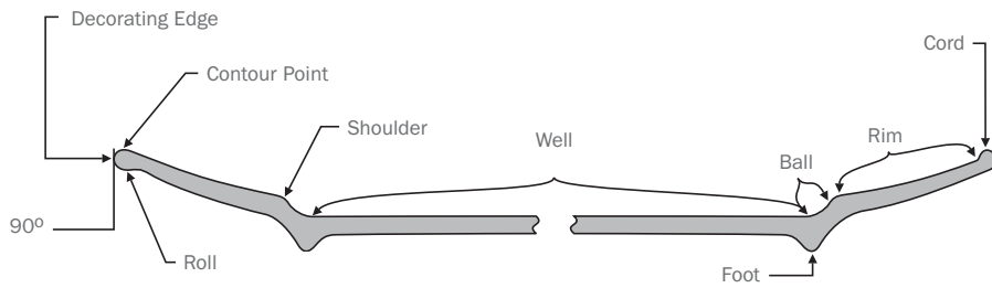
GENERIC PLATE CROSS SECTION
